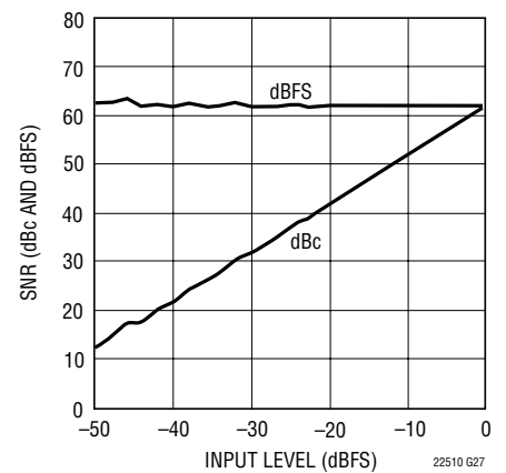
LTC2250: SNR vs Input Level, f_{IN} = 70\text{MHz} , 2V Range, 105Mpsps
