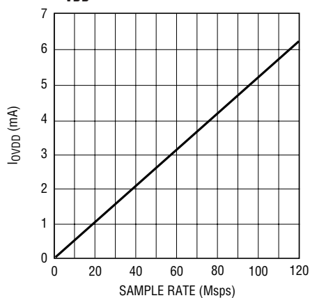
LTC2250: I_{OVD} vs Sample Rate, 5MHz Sine Wave Input, -1dB, O_{VDD} = 1.8\text{V}
