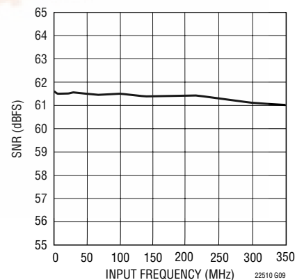
LTC2251: SNR vs Input Frequency, -1dB, 2V Range, 125MSPs
