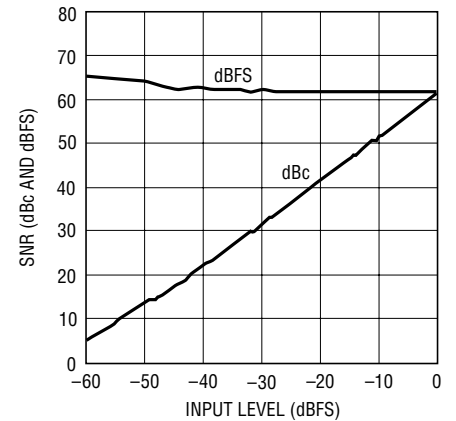
LTC2237: SNR vs Input Level, f_{IN} = 5\text{MHz} , 2V Range, 40Mps
