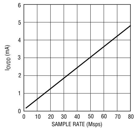
LTC2238: I_{OVD} vs Sample Rate, 5MHz Sine Wave Input, -1dB, O_{VDD} = 1.8\text{V}
