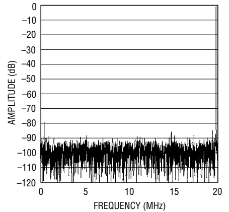
LTC2237: 8192 Point FFT, f_{IN} = 140\text{MHz} , -1\text{dB} , 2V Range, 40Mps
