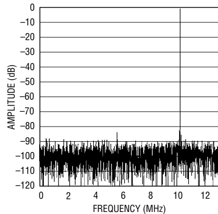
LTC2236: 8192 Point FFT, f_{IN} = 140\text{MHz} , -1dB, 2V Range, 25Mps
