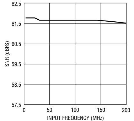
LTC2237: SNR vs Input Frequency, -1\text{dB} , 2V Range, 40Mps
