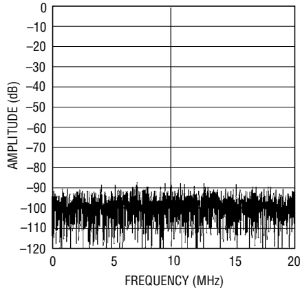
LTC2237: 8192 Point FFT, f_{IN} = 70\text{MHz} , -1\text{dB} , 2V Range, 40Mps
