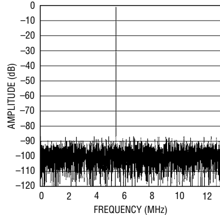
LTC2236: 8192 Point FFT, f_{IN} = 5\text{MHz} , -1dB, 2V Range, 25Mps
