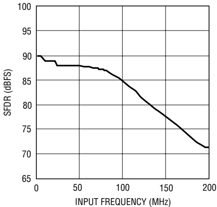
LTC2237: SFDR vs Input Frequency, -1\text{dB} , 2V Range, 40Mps
