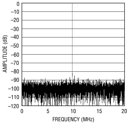
LTC2237: 8192 Point FFT, f_{IN} = 30\text{MHz} , -1\text{dB} , 2V Range, 40Mps
