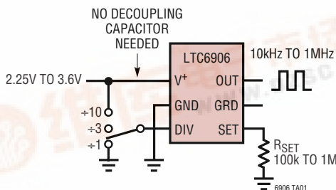
Micropower Clock Generator
