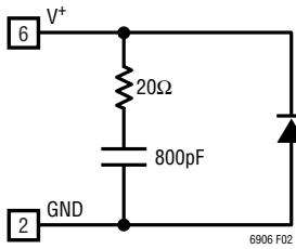
Figure 2. V+ Pin
