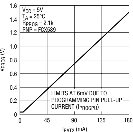
Program Pin Voltage vs Charge Current (180mA)
