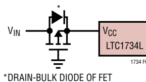
Figure 6. Low Loss Reverse Voltage Protection
