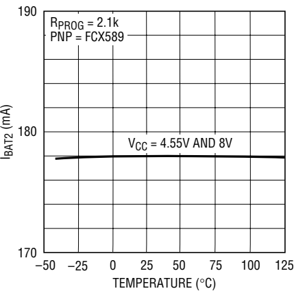
I_{BAT2} vs Temperature and Supply Voltage
