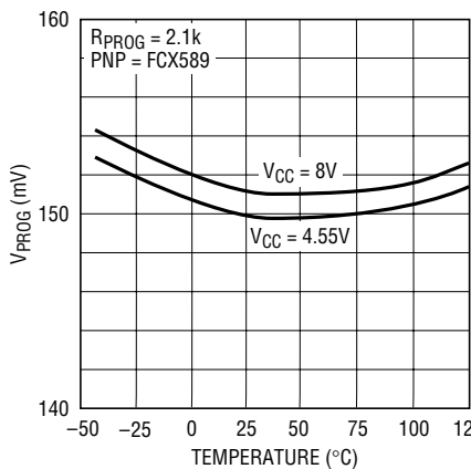
Program Pin Voltage for I_{BAT2}/10 vs Temperature and Supply Voltage
