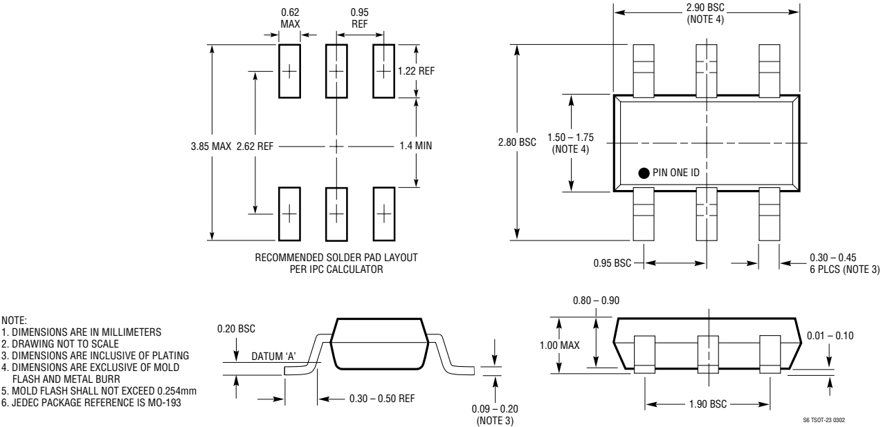
S6 Package 6-Lead Plastic TSOT-23 (Reference LTC DWG # 05-08-1636)
