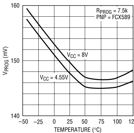
Program Pin Voltage for I_{BAT1}/10 vs Temperature and Supply Voltage
