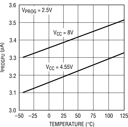
Program Pin Pull-Up Current vs Temperature and Supply Voltage
