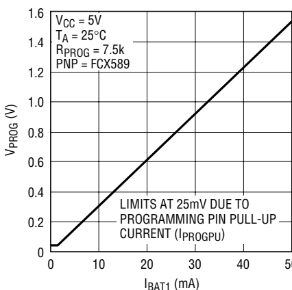
Program Pin Voltage vs Charge Current (50mA)
