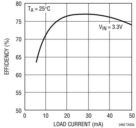
-8V Efficiency
