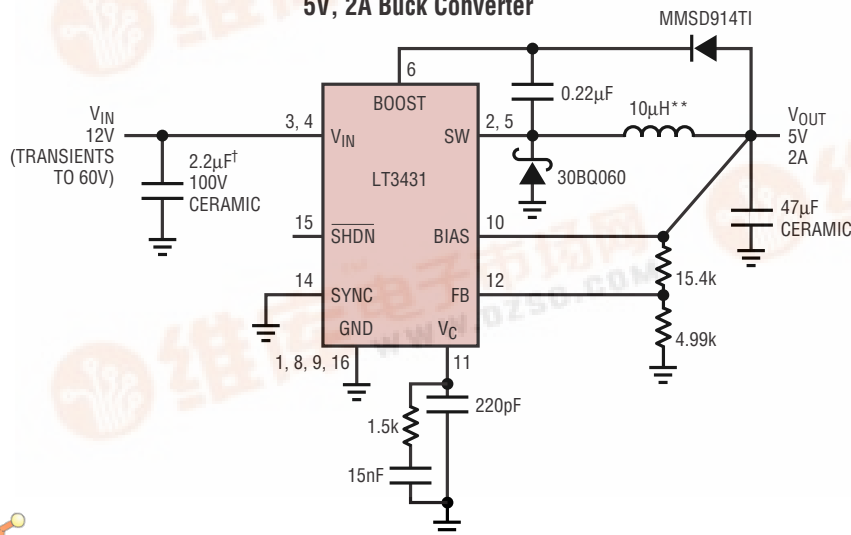
5V, 2A Buck Converter
