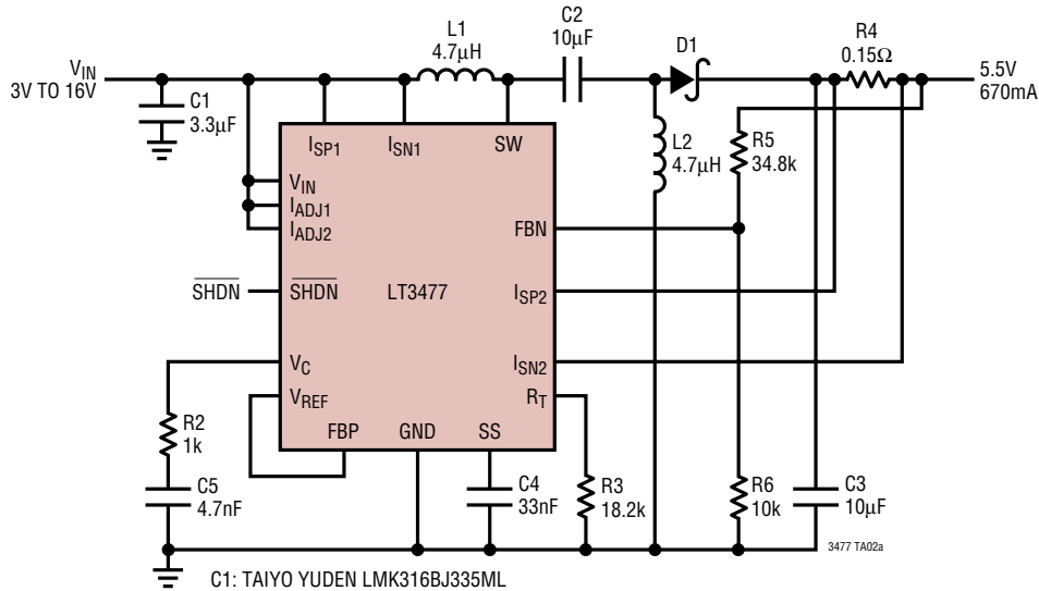
5.5V SEPIC Converter with Short-Circuit Capability
