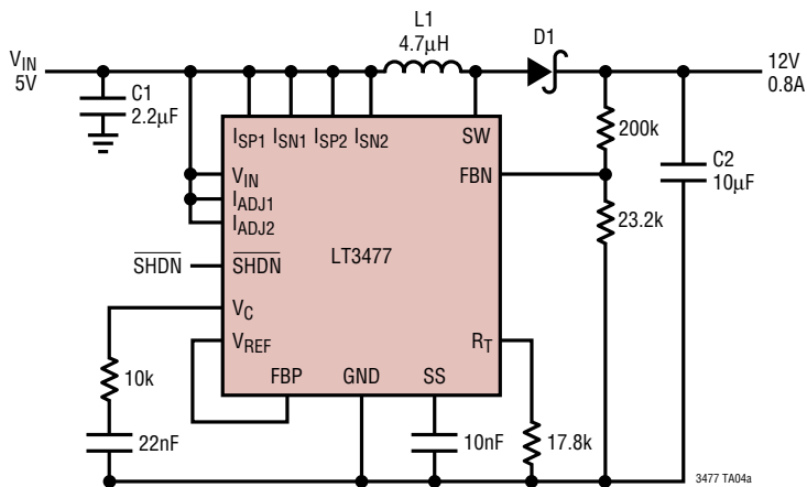
800mA, 5V to 12V Boost Converter
