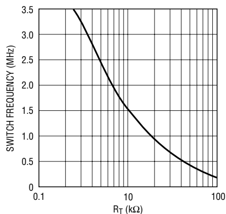
Figure 5. Switch Frequency
