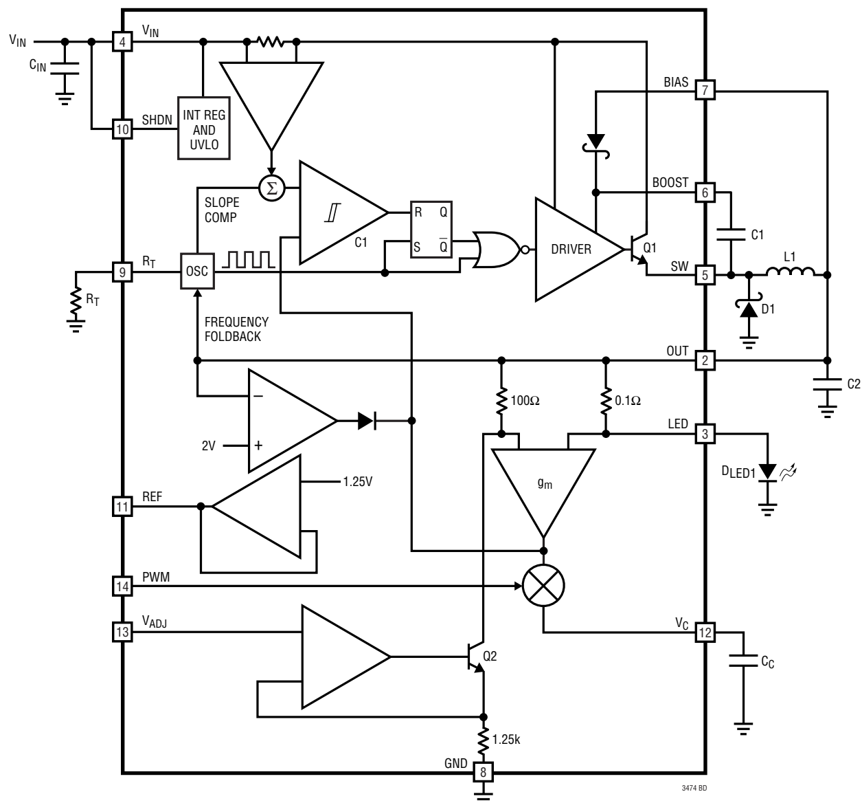
Figure 1. Block Diagram
