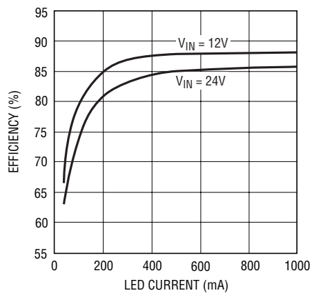
Efficiency, Two LED Output
