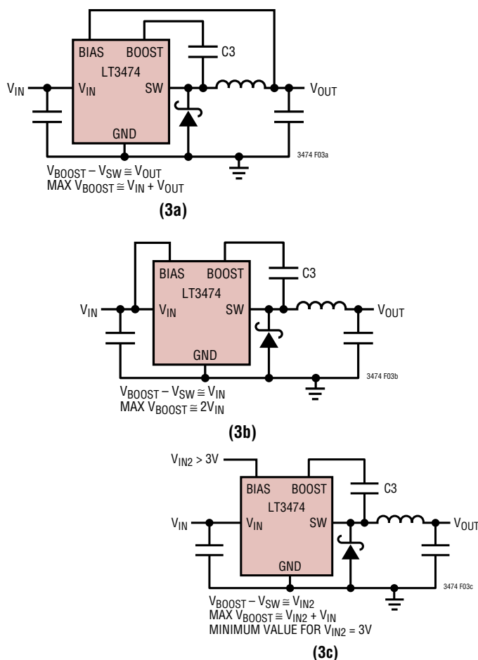
Figure 3. Generating the Boost Voltage
