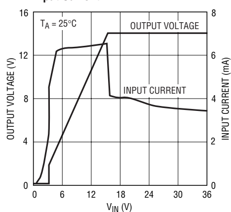
Open-Circuit Output Voltage and Input Current
