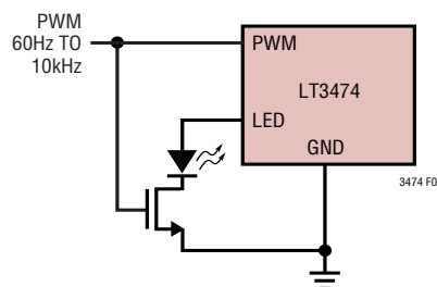
Figure 6. Dimming Using PWM Signal
