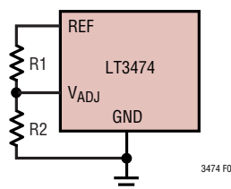
Figure 4. Setting V ADJ with a Resistor Divider
