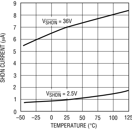
SHDN Bias Current vs Temperature
