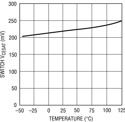
Switch V_{CESAT} ( I_{SW} = 100mA ) vs Temperature
