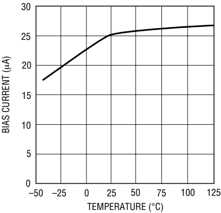
BIAS Quiescent Current (Bias > 3V) vs Temperature
