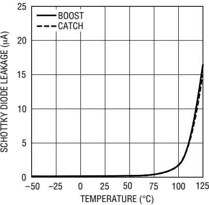
Diode Leakage ( V_R = 36V ) vs Temperature
