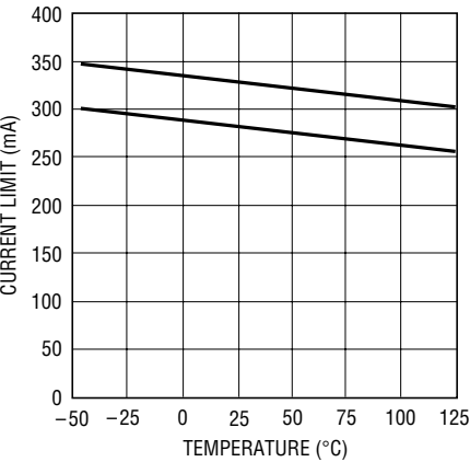
Top and Bottom Switch Current Limits ( V_{FB} = 0V ) vs Temperature
