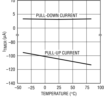
TIMER Pin Currents vs Temperature
