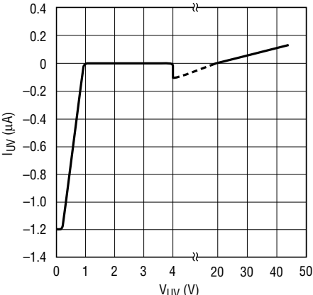
UV Pin Current vs UV Pin Voltage
