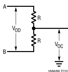
Figure 1. Driver DC Test Load
