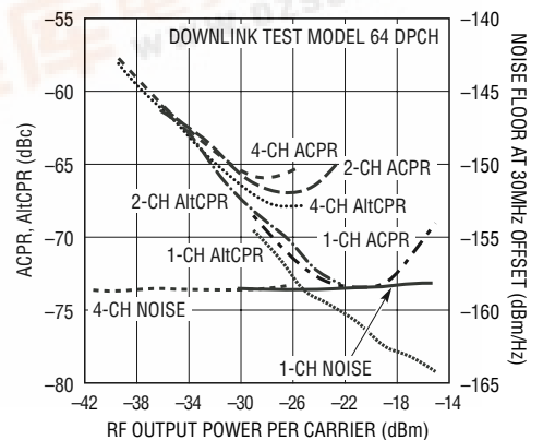
W-CDMA ACPR, AICPR and Noise vs RF Output Power at 2140MHz for 1, 2 and 4 Channels
