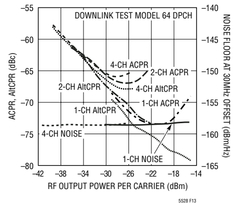
Figure 13: W-CDMA APCR, AItCPR and Noise vs RF Output Power at 2140MHz for 1, 2 and 4 Channels
