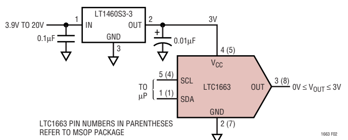
Figure 2. LT1460 As Power Supply for the LTC1663
