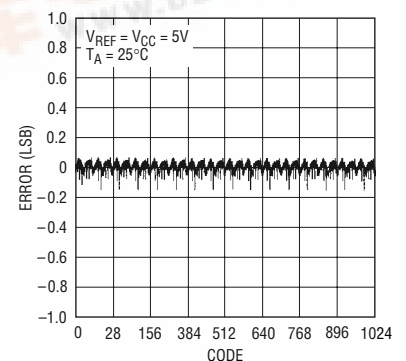
Differential Nonlinearity (DNL)
