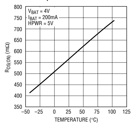
USBIN Power FET "On" Resistance vs Temperature
