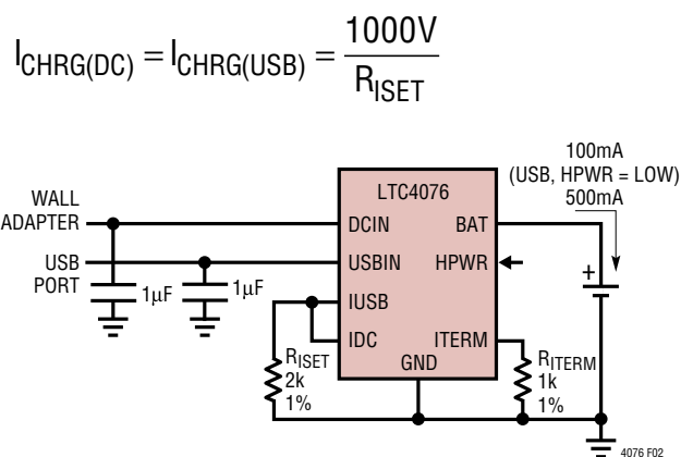
Figure 2. Dual Input Charger Circuit. The Wall Adapter Charge Current and USB Charge Current are Both Programmed to be 500mA
