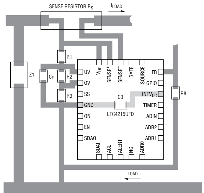
Figure 5. Recommended Layout
