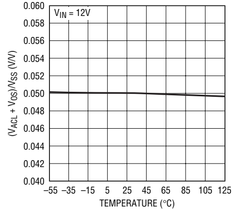
(V_{ACL} + V_{OS})/V_{SS} vs Temperature
