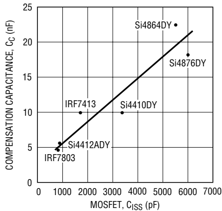
Figure 6. Recommended Compensation Capacitor C_C vs MOSFET C_{ISS}
