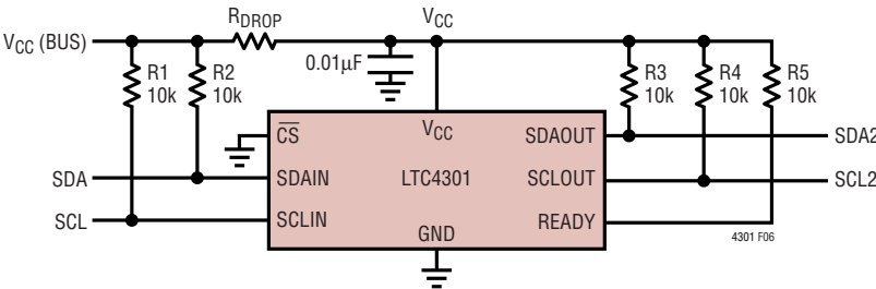
Figure 7. System with \text{V}_{\text{CC}} Voltage Droop
