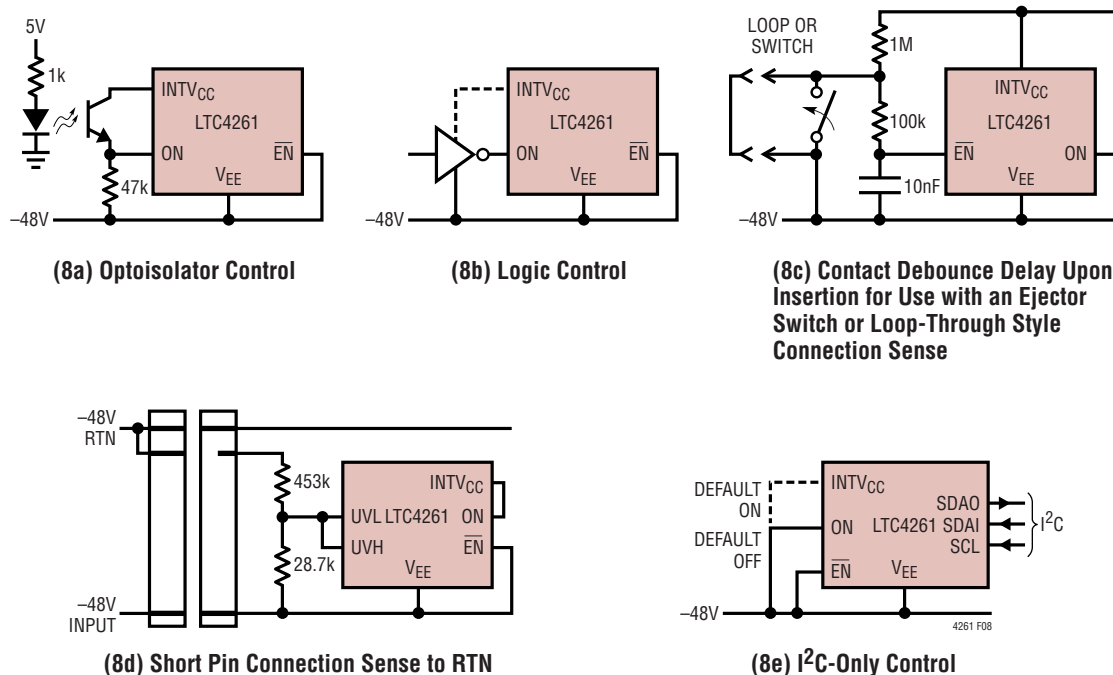
Figure 8. On/Off Control of the LTC4261
