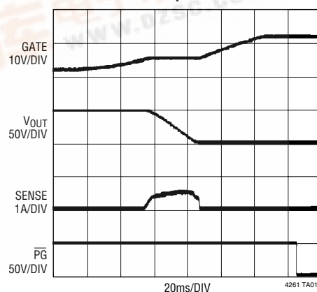
Start-Up Behavior
