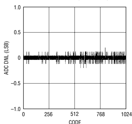
ADC DNL vs Code (ADIN Pin)
