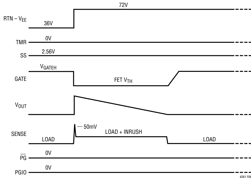
Figure 6. -36V to -72V Step Response
