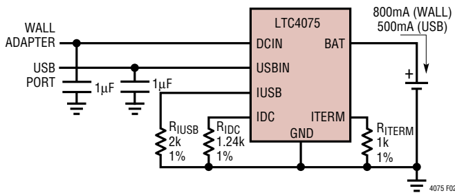
Figure 2. Full Featured Dual Input Charger Circuit
