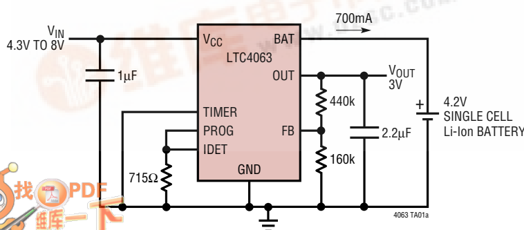
Single Cell Li-Ion Battery Charger with Regulated 3V Output (C/10 Termination)
