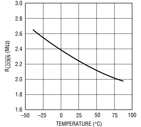
LDOEN Pin Pull-Down Resistance vs Temperature
