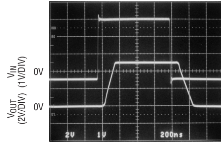
Output-Overdrive Recovery
