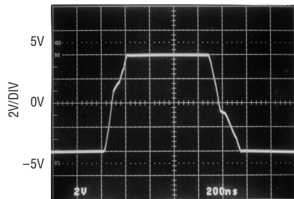
\pm 5V Large-Signal Response
