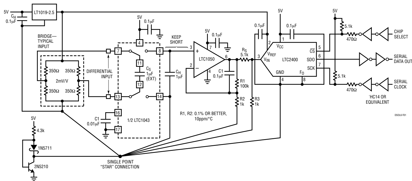
Figure 6. Single Supply Differential to Single-Ended Converter for Low Level Inputs with "Live at Zero" Operation
