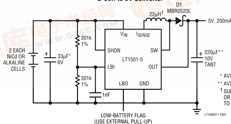
2-Cell to 5V Converter
