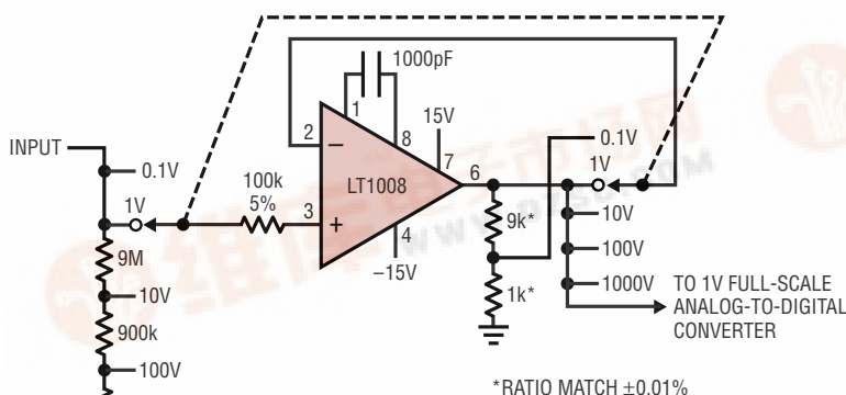
Input Amplifier for 4.5 Digit Voltmeter
