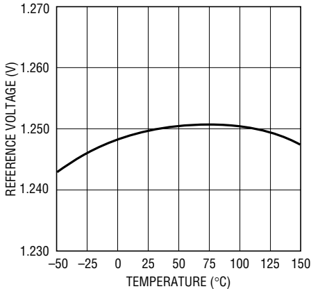
Temperature Stability
