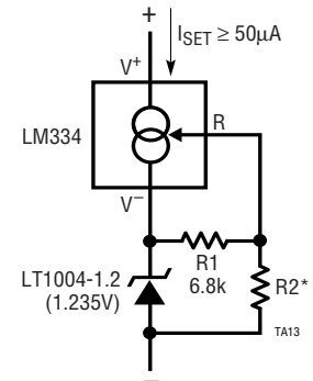
High Precision Low TC Current Source
