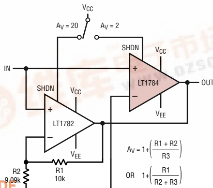
Programmable Gain, A v = 2, A v = 20, 100kHz Amplifier
