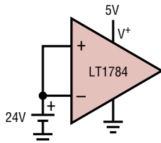
INPUT OVERVOLTAGE
