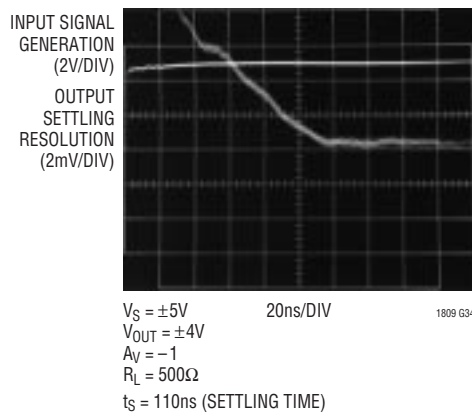
0.01% Settling Time
