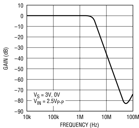
Figure 11. Filter Frequency Response
