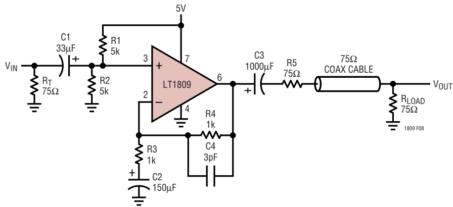
Figure 8. 5V Single Supply Video Line Driver
