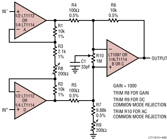
Three Op Amp Instrumentation Amplifier
