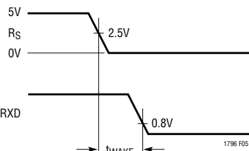
Figure 5. Wake Up from Standby Waveforms
