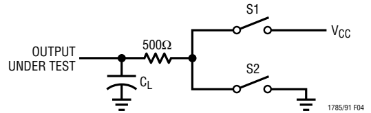
Figure 4. Driver Timing Test Load
