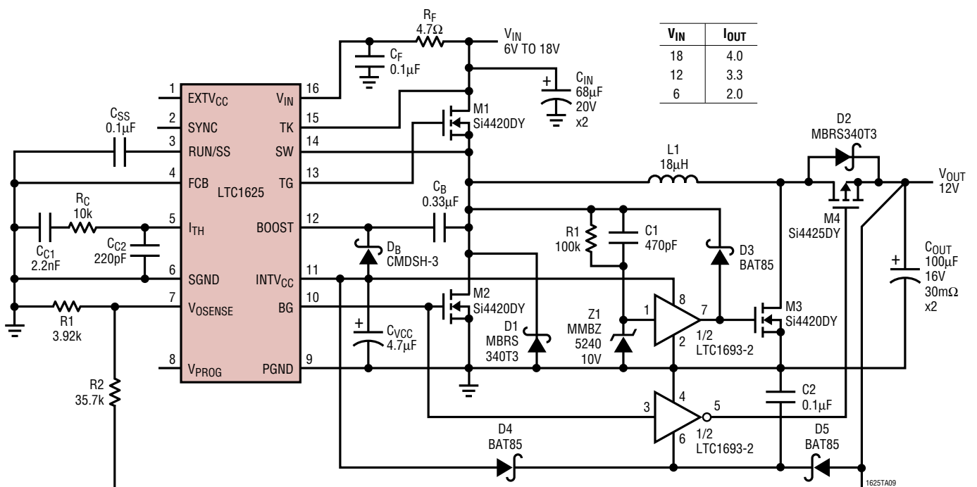
Single Inductor, Positive Output Buck Boost
