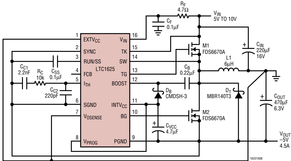
-5V/4.5A Positive to Negative Converter
