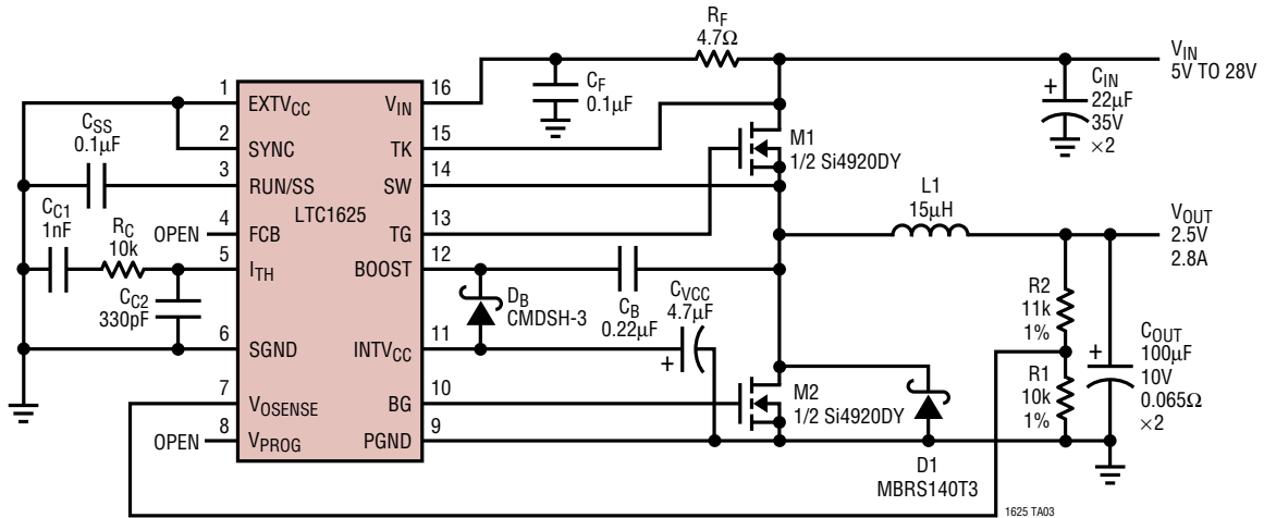
2.5V/2.8A Adjustable Output
