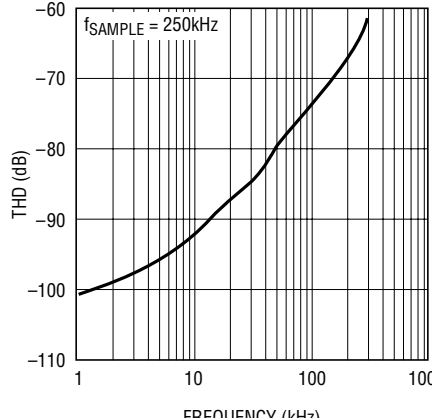
Total Harmonic Distortion (THD) vs Input Frequency
