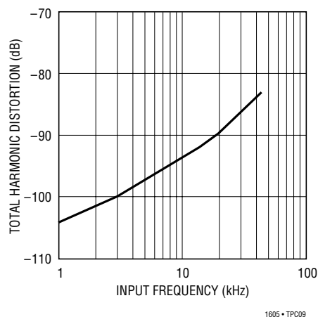
Total Harmonic Distortion vs Input Frequency
