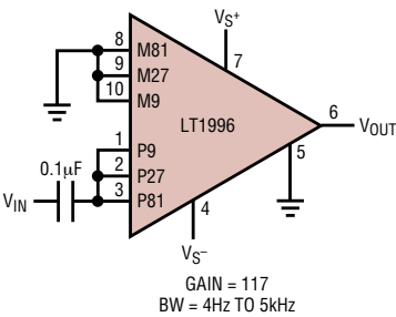
AC Coupled Amplifier
