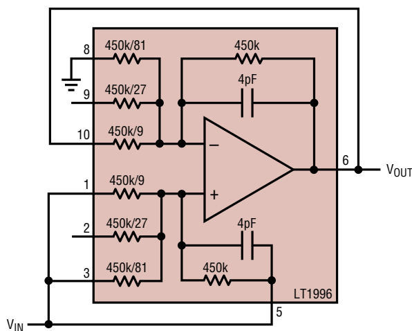
CLASSICAL NONINVERTING OP AMP CONFIGURATION IMPLEMENTED WITH LT1991. R_F = 45k , R_G = 5.6k , GAIN = 9.1.
