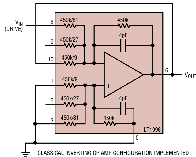
CLASSICAL INVERTING OP AMP CONFIGURATION IMPLEMENTED WITH LT1991. R_F = 45k , R_G = 5.55k , \text{GAIN} = -8.1 .
