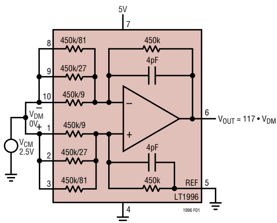
Figure 1. Difference Amplifier Cannot Produce 0V on a Single Supply. Provide a Negative Supply, or Raise Pin 5, or Provide 400μV of V_{DM}
