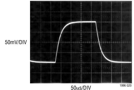
Small Signal Transient Response, Gain = 81
