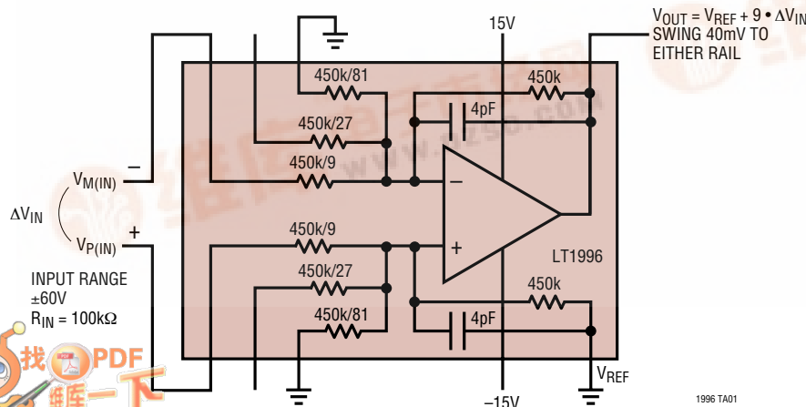
Rail-to-Rail Gain = 9 Difference Amplifier
