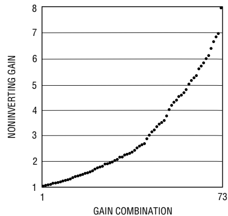
Figure 4. Unique Noninverting Gain Configurations
