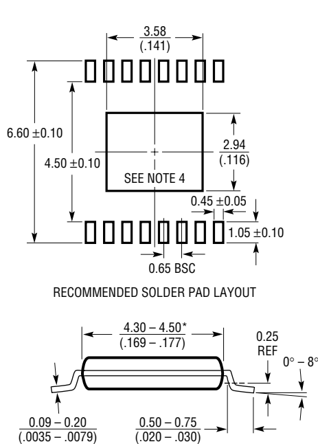
FE Package 16-Lead Plastic TSSOP (4.4mm) (Reference LTC DWG # 05-08-1663) Exposed Pad Variation BC
