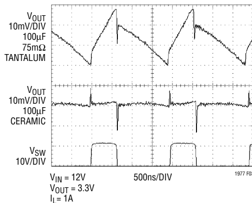
Figure 3. LT1977 Ripple Voltage Waveform
