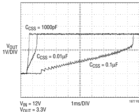
Figure 4. V_{OUT} dV/dt
