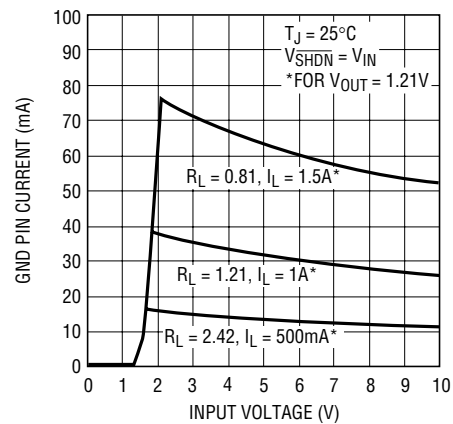
LT1963A GND Pin Current
