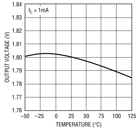
LT1963A-1.8 Output Voltage
