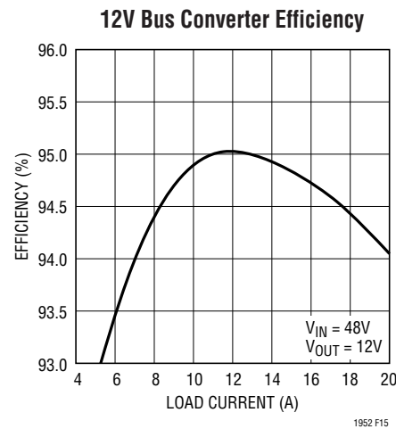
Figure 15. LT1952-Based Synchronous 'Bus Converter' Efficiency vs Load Current (For Circuit in Figure 16)
