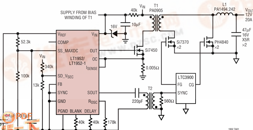
36V to 72V Input, 12V at 20A Semi-Regulated Bus Converter
