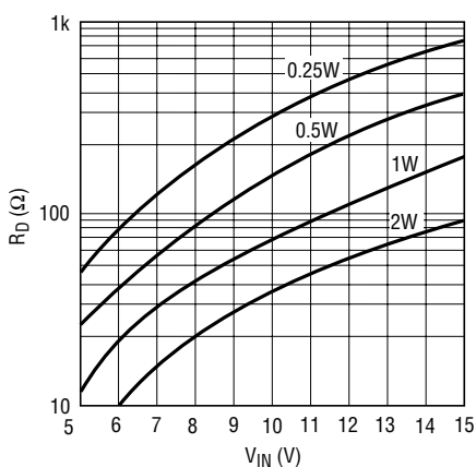
Figure 8. Power in R_D
