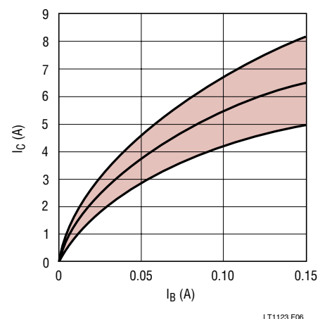
Figure 6. MJE1123 I_C vs I_B
