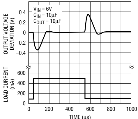
LT1763-5 Transient Response C_{BYP} = 0
