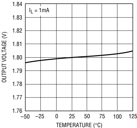
LT1763-1.8 Output Voltage
