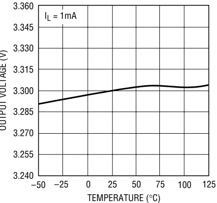
LT1763-3.3 Output Voltage
