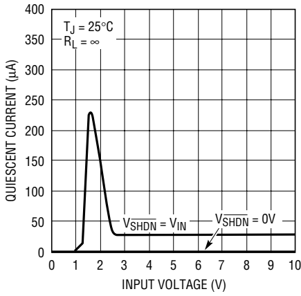
LT1762-2.5 Quiescent Current
