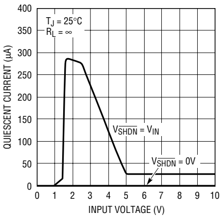
LT1762-5 Quiescent Current
