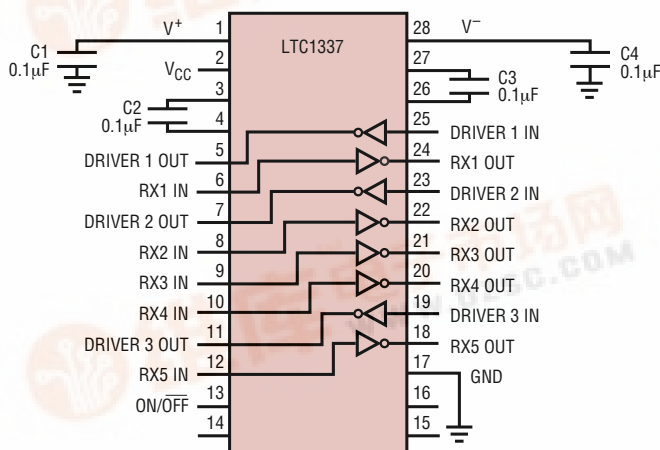
3-Drivers/5-Receivers with Shutdown
