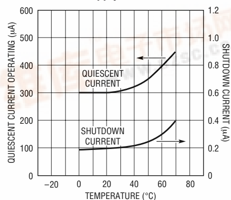
Supply Current
