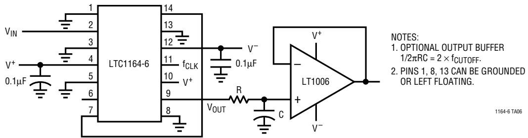
8th Order Elliptic Lowpass Filter ( f_{CLK}/f_C ) = 50:1
