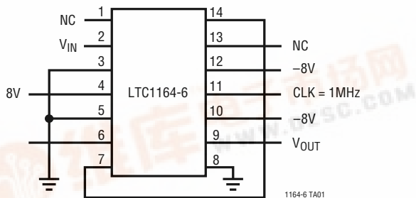
10kHz Anti-Aliasing Elliptic Filter
