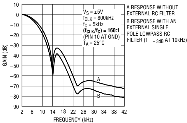
Stopband Gain vs Frequency (Linear Phase Response)
