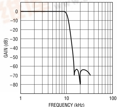
Frequency Response
