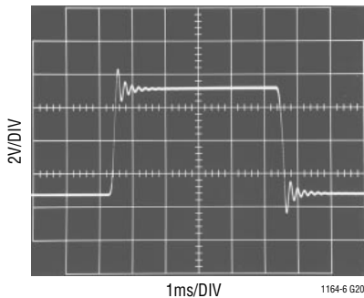
Transient Response
