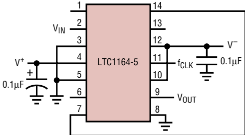
8th Order Butterworth Lowpass Filter f_{CLK}/f_C = 100:1
