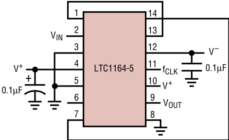
8th Order Butterworth Lowpass Filter f_{CLK}/f_C = 50:1
