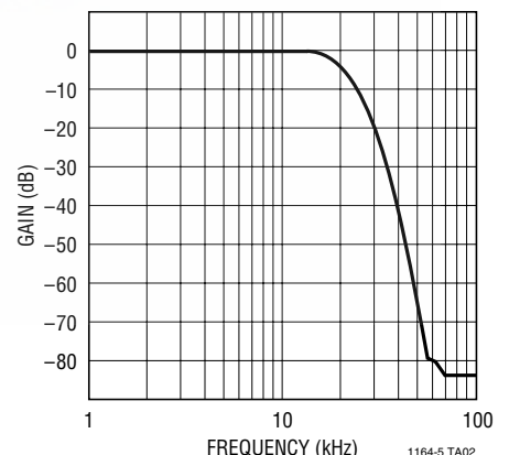
Frequency Response
