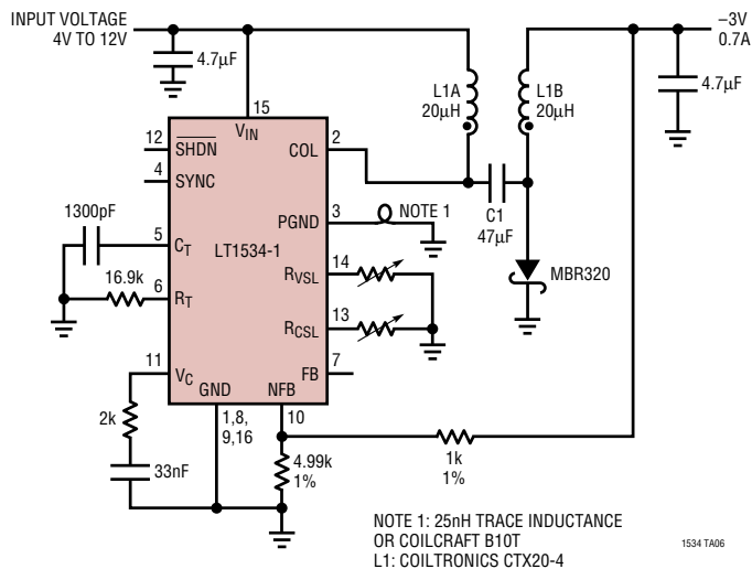
Ultralow Noise 5V to -3V Cuk Converter
