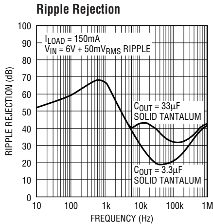
LT1521 • TPC31
