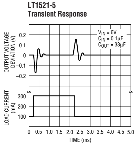
LT1521 • TPC34
