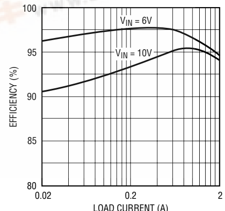
LTC1148-5 Efficiency
