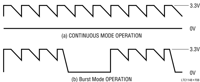
Figure 8. C_T Waveforms
