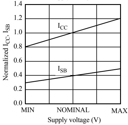
Normalized supply current I_{CC} , I_{SB} vs. supply voltage V_{CC}
