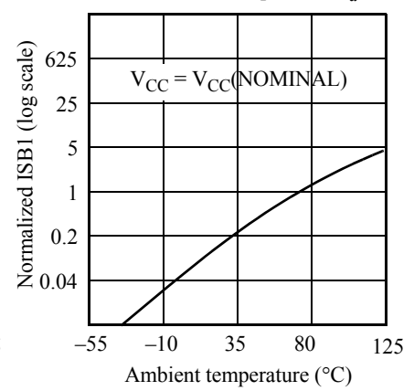
Normalized supply current I_{SB1} vs. ambient temperature T_a
