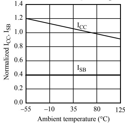
Normalized supply current I_{CC} , I_{SB} vs. ambient temperature T_a
