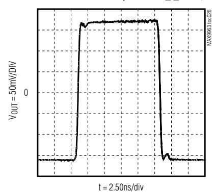
COMPARATOR DIFFERENTIAL OUTPUT RESPONSE, MAX996_GCCQ
